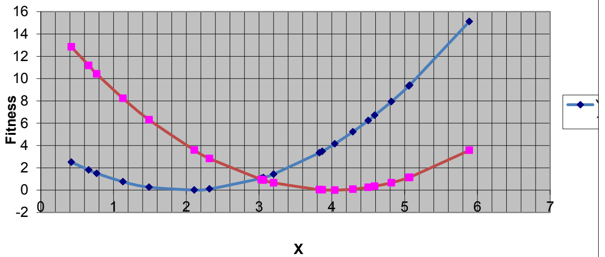
Gen 1 - Fitness
