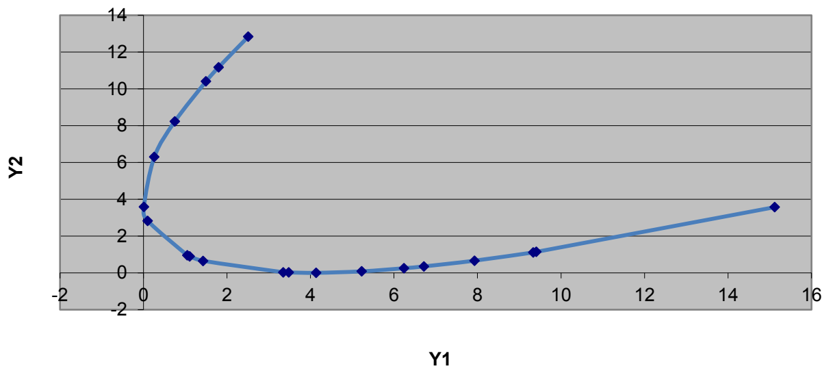
Gen 1 Ranking
