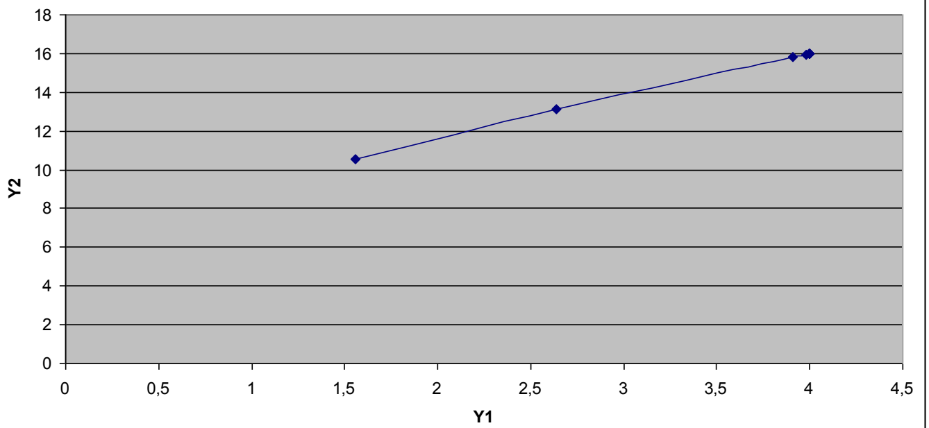
Gen 10 Ranking
