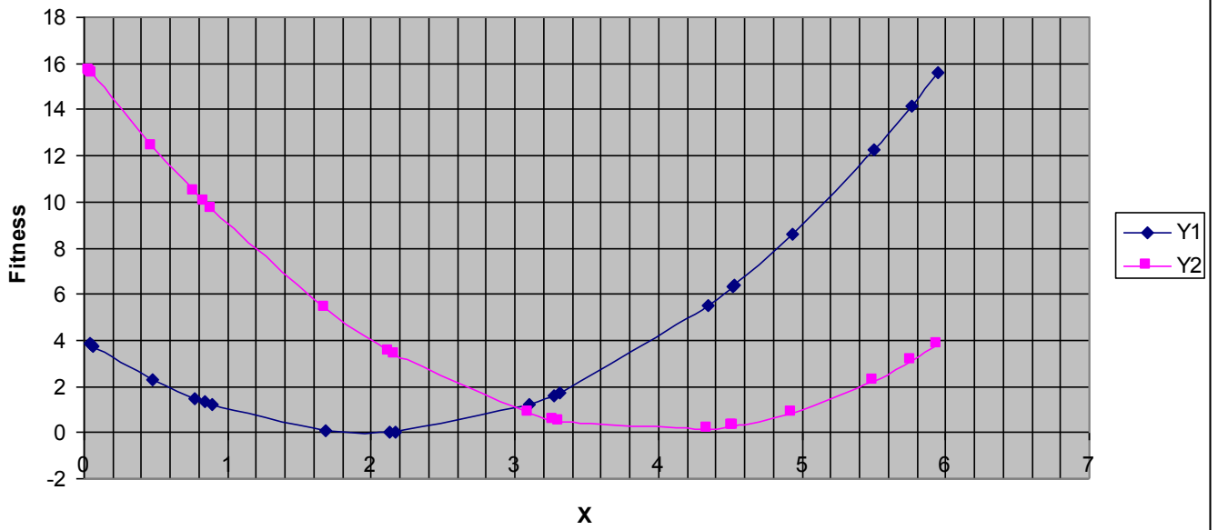
Gen 1 Ranking
