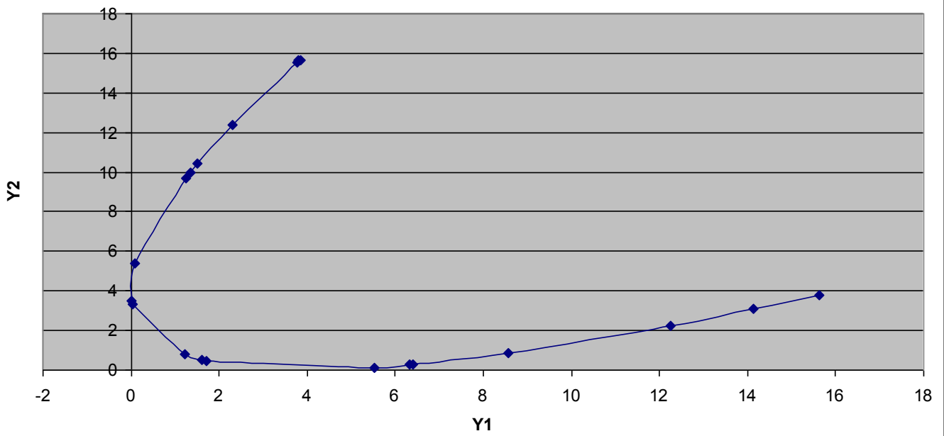
Gen 1 Ranking
