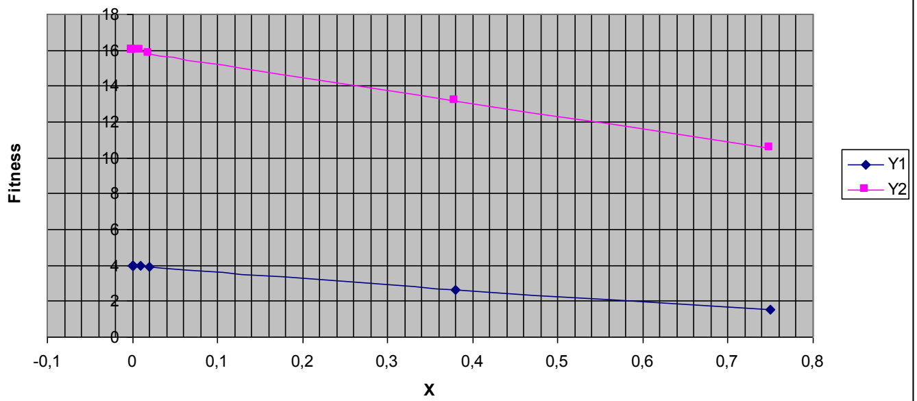
Gen 10 Ranking
