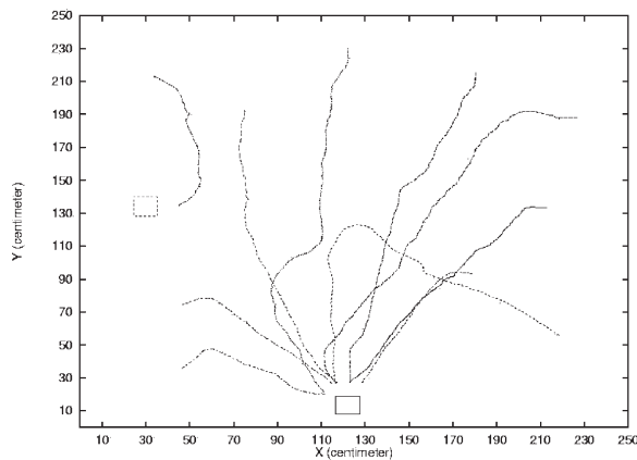
Fig. 8. The behavior of the robot when played two simultaneous calling songs with different carrier frequencies. The lower box is a speaker playing a 4.7 kHz song, which matches the time delays used in the peripheral auditory processing. The left box is a speaker playing a 6.7 kHz song. Each line is a separate trial, with the robot starting from 10 different positions in the arena. It always successfully approaches a sound source; only once is this the song with the wrong carrier frequency.
