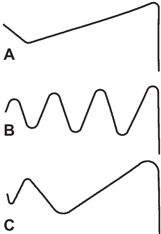
Fig. 16. Examples of robot tracking performances with algorithm settings emphasizing speed to the source, but not source location (A); source location, but not speed to the source (B); and intermediate strategy (C) achieved by modulating the turn magnitude and crosswind steering angle with local plume concentration. Wind in this figure is blowing from left to right.
