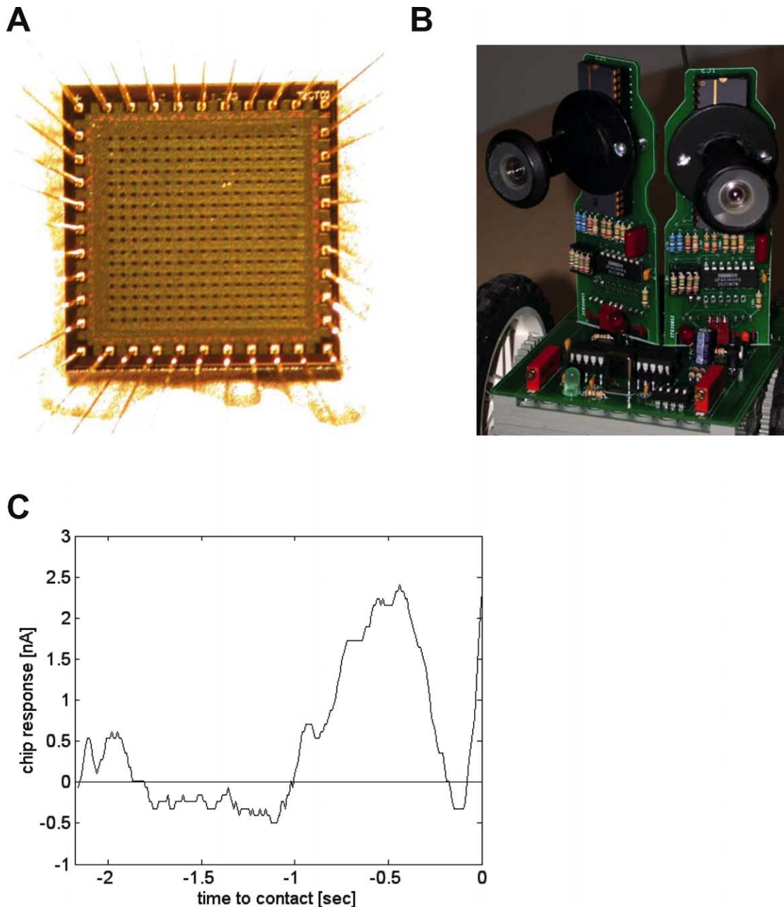
Fig. 4. A. Collision detector chip measuring 2.2\text{ mm} \times 2.2\text{ mm} . The chip contains a 17 \times 17 array of photoreceptors with motion detectors between neighboring cells. The chip consumes 140\text{ }\mu\text{W} of power. B. Small robotic vehicle with two collision detector chips mounted behind wide-angle lenses (black structures). For scale the round lens housings are 2.5 cm in diameter. C. Measured output of collision detection chip after off-chip leaky integration. The peak response of the chip occurs approximately 500 ms before contact, which corresponds to a distance of 14 cm from the obstacle.
