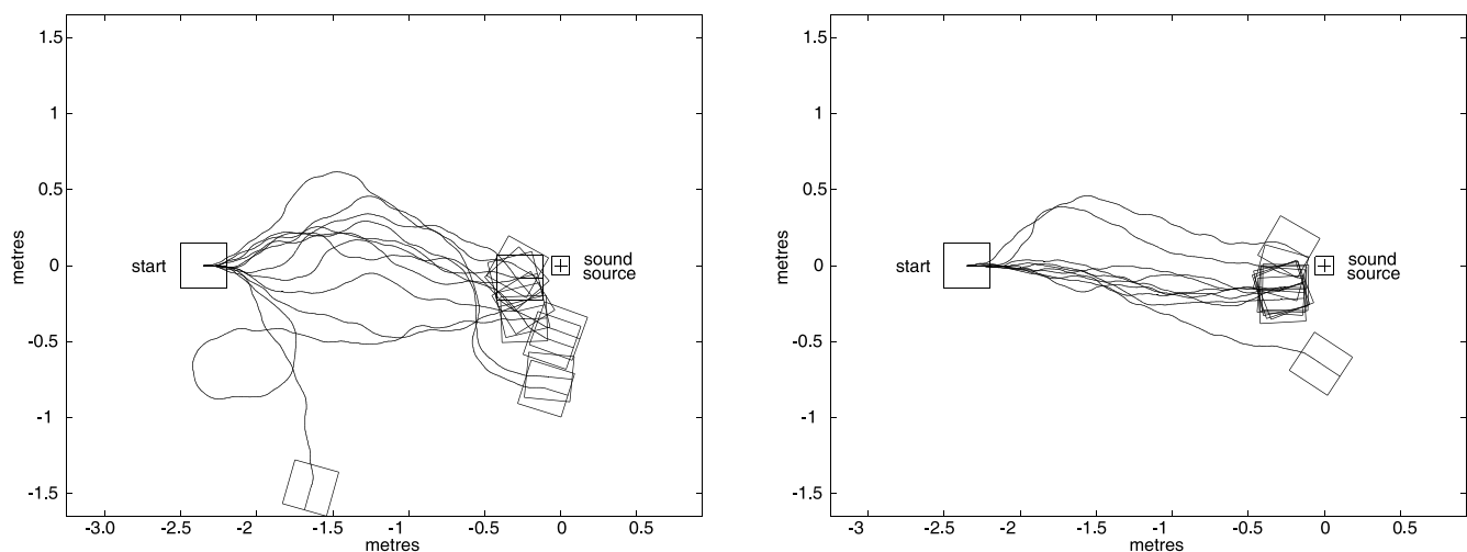
Fig. 11. Tracks of the robot to a cricket song when it has an imposed bias to rightward motion. Left, phonotaxis alone is not always sufficient to overcome the bias and the robot misses the sound source. Right, with an optomotor system also active, the robot is able to track more directly to the sound source.
