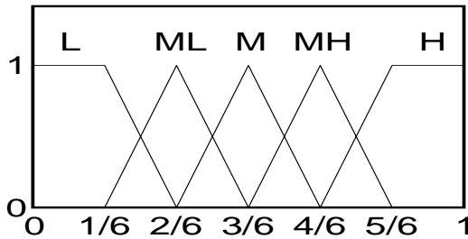
Fig. 2. Five fixed shaped membership functions each of which describes how likely a coordinate is either Low (L), Middle-Low (ML), Middle (M), Middle-High (MH), or High (H). Note that the coordinates in [-1, 1] are translated into [0, 1] with interpretation being intact.
