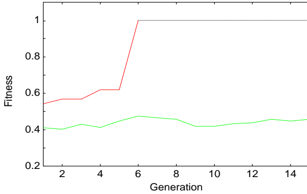
Fig. 4. Evolution to find the island in the 6-dimensional lake. Upper plot is when x_i \in [0.25, 0.75] and lower plot is for a small island where x_i \in [0.45, 0.55] ( i = 1, \dots, 6 ).
