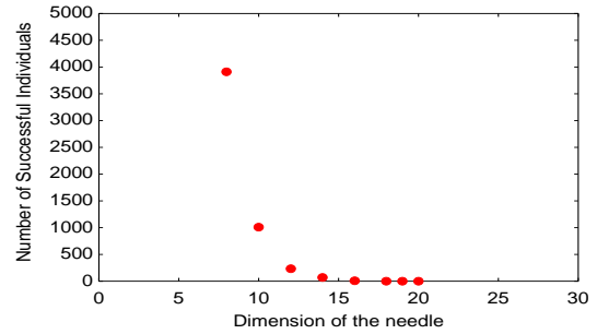
Fig. 3. The number of happened-to-be-the-needle out of 5000 random creations of the candidate.
