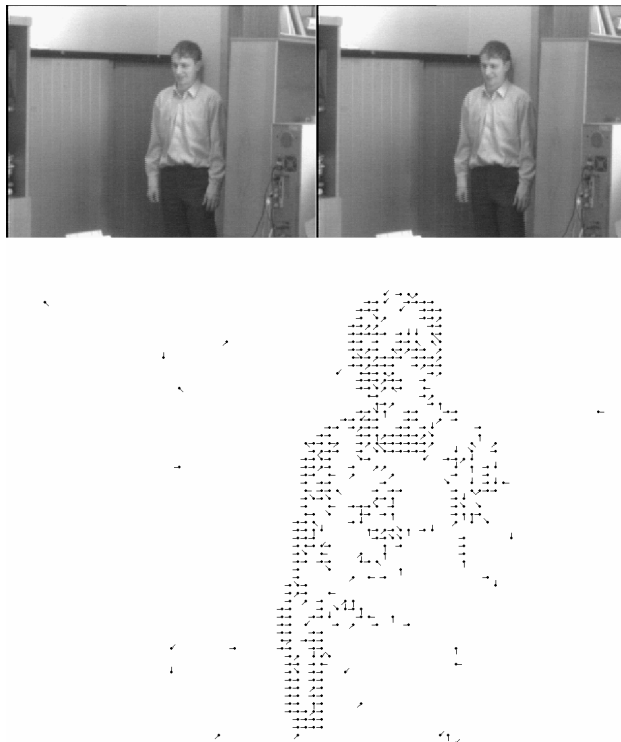
Fig. 3. Optical flow estimation procedure result.
