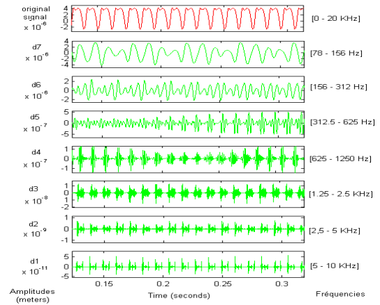
Figure 2: Wavelet decomposition of a vibratory signal corresponding to flaking path defect (depth 157µm) at speed of 1500 rpm with wavelet sym7.
