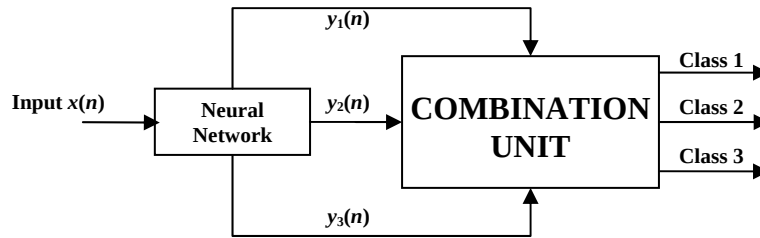
Figure 4: Single-Expert ANN based classifier.
