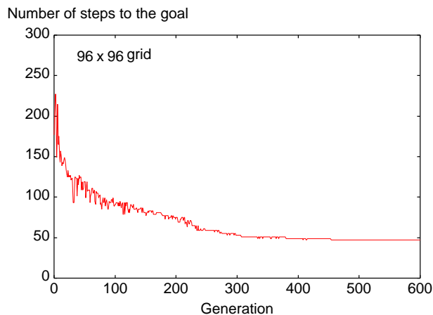
Figure 1: Fitness vs. generation.
