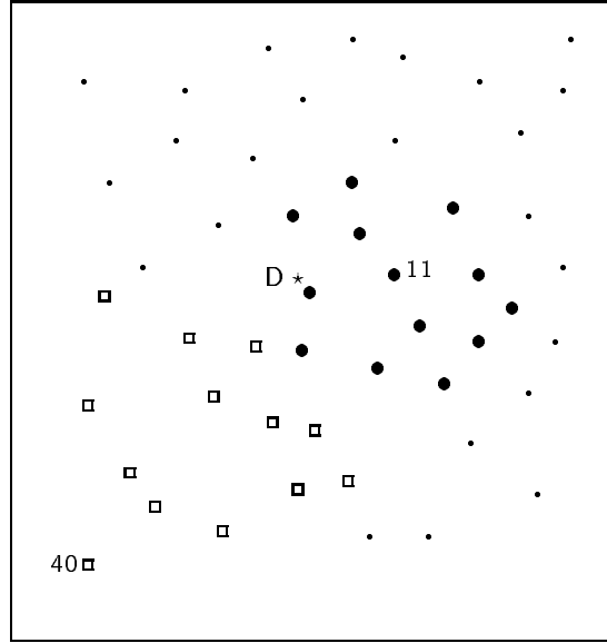
Figure 2. 50-Customer Problem (C1) with two Candidate Sets
