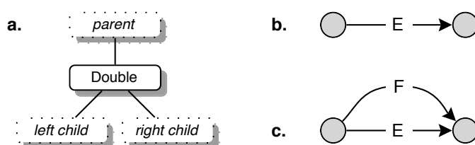
Figure 23 The double Edge Encoding operator.
