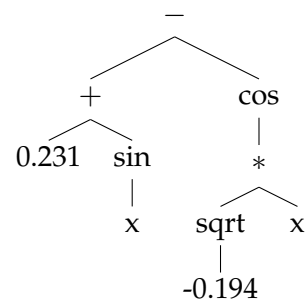
Figure 21 The tree in Figure 20 with ERC placeholders replaced with permanent constants.
