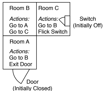
Figure 66 A robot world with three rooms, a door, and a switch. available actions for each room are shown. The robot can only exit if the door is closed. Flicking the switch opens the door.
