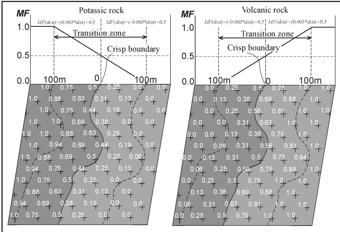
Figure 2 – Exemplars of fuzzy members on a transition zone between the lithological units, potassic rock (dark gray) and volcanic rock (light gray).
