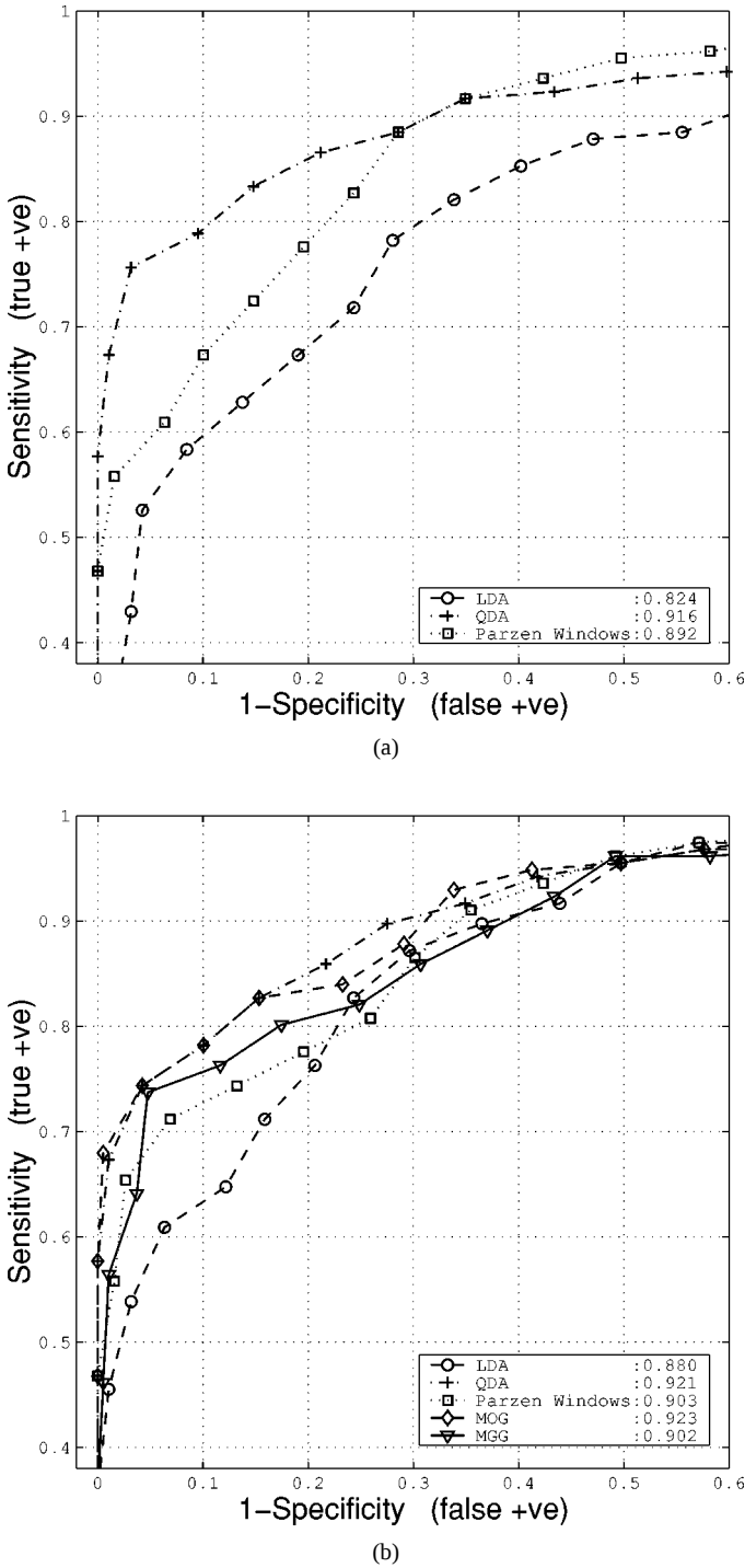
Fig. 6. ROC curves for the generative classifiers on (a) full-dimension and (b) PCA-reduced dimension data.
