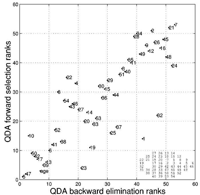
Fig. 9. Correlation of rankings given by forward selection and backward elimination on the variables (52 visual-field locations + Age). Variables close to origin (e.g., location 5 and 47, etc.) are more informative in glaucoma diagnosis. Lower right insert displays the relative positions on the retina of the variables.
