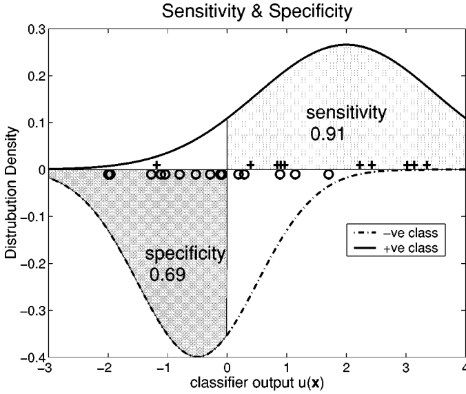
Fig. 4. Sample distribution of classifier output u(\mathbf{x}) on a two classes dataset.
