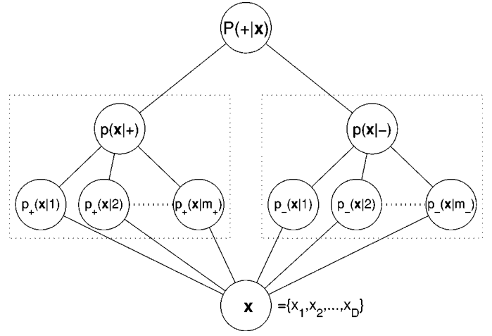
Fig. 2. Architecture of the MOG used in a binary classification setting, p(\mathbf{x}|\pm) are the generative models for the two classes. Each is composed of a MOGs [ p_+(\mathbf{x}|m_+) or p_-(\mathbf{x}|m_-) ]. Output P(+|\mathbf{x}) is obtained by applying Bayes' rule (1) on p(\mathbf{x}|\pm) .
