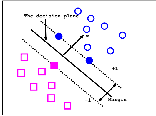
Fig. 4. An illustration of the Support Vector Machine
