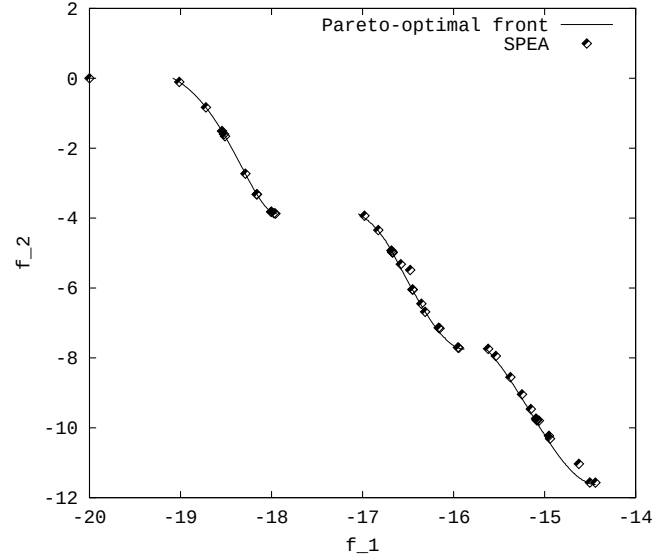
Fig. 8. Non-dominated solutions with SPEA on KUR.
