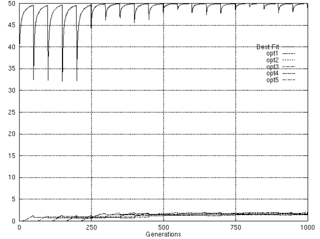
Figure 1: YaSais / Cyclic Pattern Tracking Top: best fitness, Bottom: 5 optima's densities
