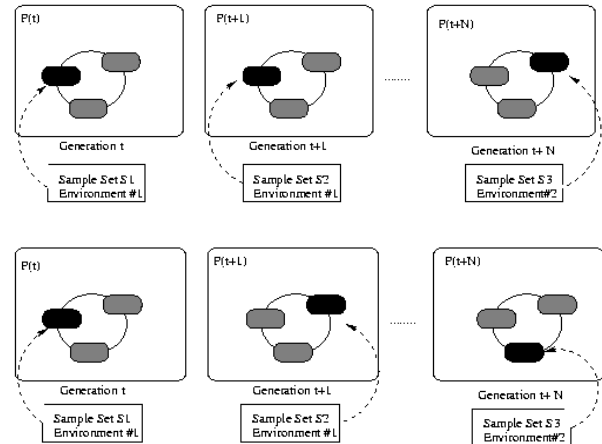
Figure 5: CLOE: specialization of B-Cells
