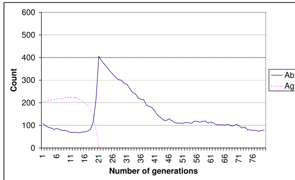
Figure 2: In combination with the residual antigen model, the memory cell model is better able to maintain a stable population of memory cells.
