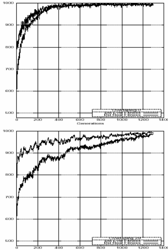
Figure 6: PICS / S-7-MUX New Evaluation Scheme (overlap parameter)
