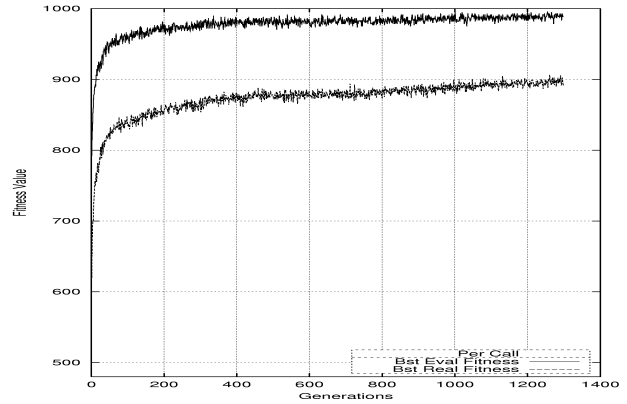
Figure 3: PICS / S-7-MUX
