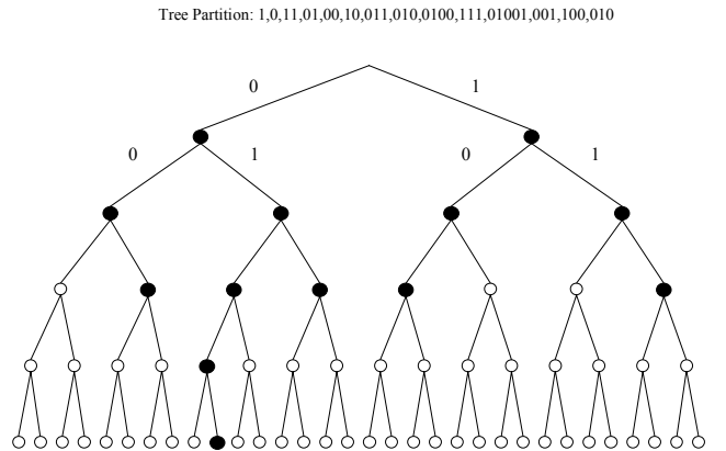
Figure 2: LZ78 binary tree representation of the partition for the binary string: 1011010010011010010011101001001100010. Nodes contained in the partition are colored in black.
