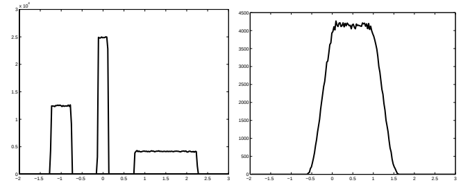
Fig. 8. 3 inputs with uniform uncertainty, but different centers and width, after convolution give semi-quadratic soft trapezoidal uncertainty distribution.
