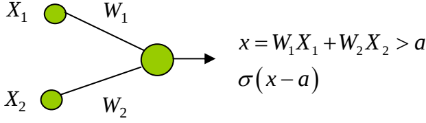
Fig. 7. Two independent inputs and one hidden neuron implementing threshold logic.
