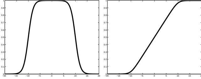
Fig. 5. Soft trapezoidal uncertainty centered at x = 0 with b = 5 , and the log-exp membership function.
