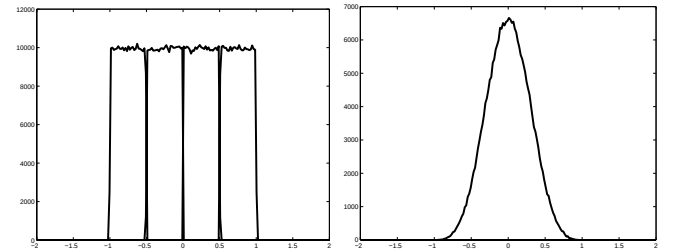
Fig. 9. 4 inputs with uniform uncertainty and identical width, centered at \pm 0.25 and \pm 0.75 , after convolution giving Gaussian-like uncertainty distribution.
