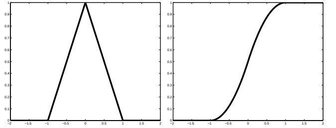
Fig. 2. Triangular uncertainty and the semiquadratic membership function that results from its integration.
