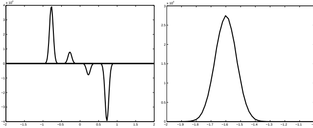
Fig. 10. 4 inputs with Gaussian uncertainty, identical dispersions, centered at \pm 0.25 and \pm 0.75 , with 1, 0.2, -0.2, -1 weights, after convolution give Gaussian-like uncertainty distribution.
