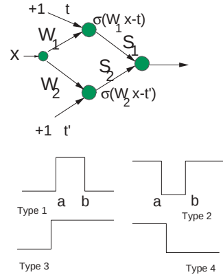
Fig. 6. Neural implementation of 4 types of crisp conditions Wx \in (a, b) , with S_1 = -S_2 = 1 and \sigma(\cdot) with infinite slopes: type 1 for W_1 = W_2 = 1 , t = a , t' = b , type 2 for W_1 = -1 , W_2 = 1 , t = -a , t' = b , type 3 is obtained from type 1 with b = \infty and type 4 is obtained from type 2 with b = -\infty .
