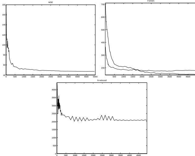
Fig. 4. Convergence of the same network with dynamic \epsilon threshold determination: upper left – MSE, upper right – training (upper) and test (lower curve) accuracy; bottom, number of support vectors.
