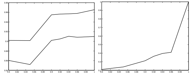
Fig. 3. Convergence of a network with 36 hidden neurons on the Satellite Image data for different thresholds \epsilon : left, training (upper) and test (lower curve) accuracy; right, number of support vectors.
