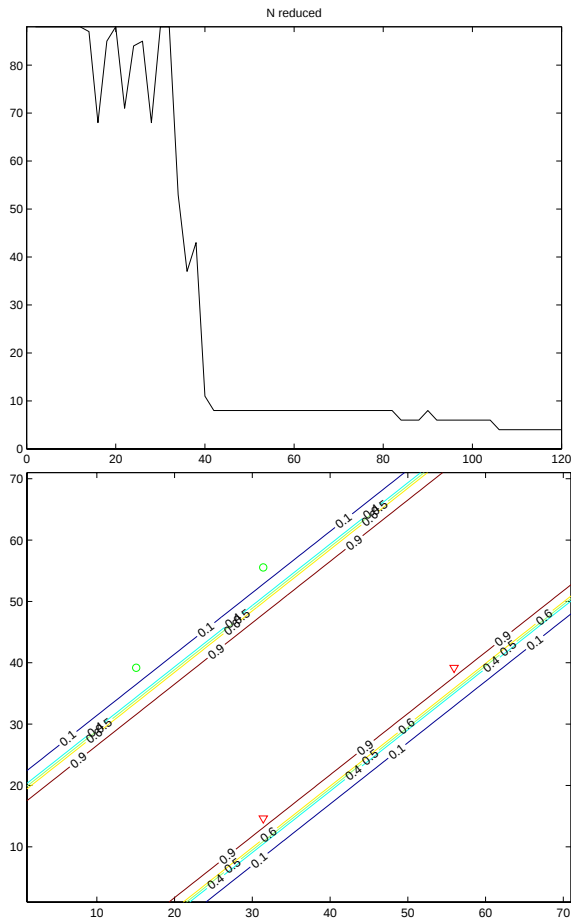
Fig. 2. Typical run on the noisy XOR data; left, the number of support vectors decreasing during iterations; right, the final solution with only support vectors shown.
