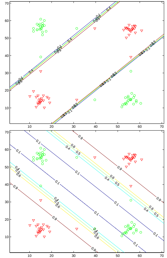
Fig. 1. Noisy XOR data with additional 8 vectors added to enforce unique borders; two perfect solutions to this problem, the lower one with wider margin achieved by adding regularization term.
