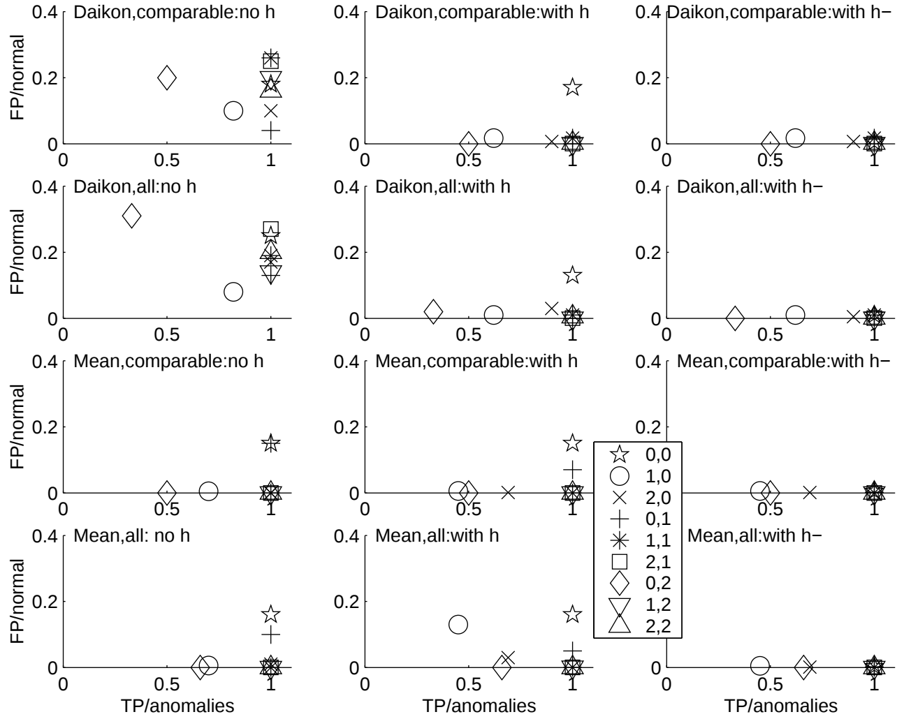
Figure 5.3: TP (True Positives) ratio vs. FP (False Positives) ratio. Best possible result: (TP/anomalies, FP/normal) = (1, 0) . Each data feed is indicated by a single marker denoted in the legend by i, j , corresponding to S_i, Q_j . Rows 1–2 depict results for Daikon, rows 3–4 for Mean. For each of Daikon/Mean, first row is the comparable-attrs variant, second row is all-attrs. First column is results without heuristic (h); second with h; third with h, after manually removing attributes that seem to be computed differently by the different data sources (h-).
