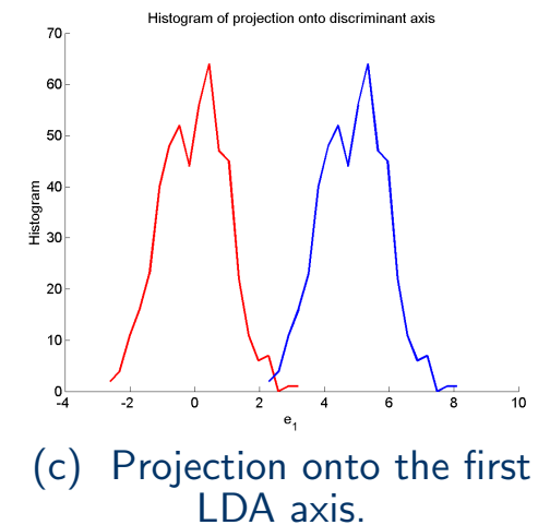
Figure 8: Scatter plot and the PCA and LDA axes for a bivariate sample with two classes. Histogram of the projection onto the first LDA axis shows better separation than the projection onto the first PCA axis.
