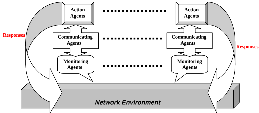
Figure 1. Conceptual view of the proposed multi-agent intrusion detection system.
