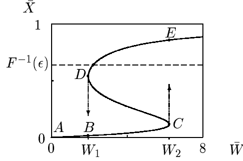
Figure 1: Hysteresis. Equilibrium manifold of \bar{X} ( \frac{d\bar{X}}{dt} = 0 ) as depending on \bar{W} ( \bar{W} = \frac{1}{N} \sum_{i,j} W_{ij} ), according to eqn(7) (states on CD are unstable with respect to \bar{X} , the others are stable). At the intersection point with the line \bar{X} = F^{-1}(\epsilon) ( F^{-1} is the inverse of F ), \bar{W} remains constant; above and below that line, it decreases and increases, respectively (see eqn(5)). Connectivity is quasi-stationary on the time scale of membrane potential dynamics, and, starting at A , \bar{X} will follow the branch ABC , until it reaches C , where it jumps to the upper branch, thus exhibiting a transition from quiescent to activated state. If the equilibrium point is on DE , \bar{W} decreases again, and a developing network has to go through a phase in which \bar{W} is higher than in the final situation, thus exhibiting a transient overshoot in \bar{W} . An intersection point on CD results in regular oscillations that follow the path ABCEDBCEDBC...
