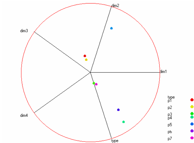
Figure 15 Simple Seven - Radviz -using Type as a Dimension
