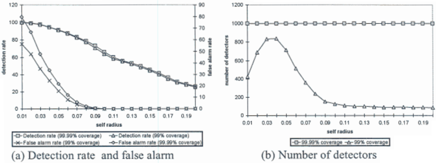
Fig. 5. Results on cross-shaped self region
