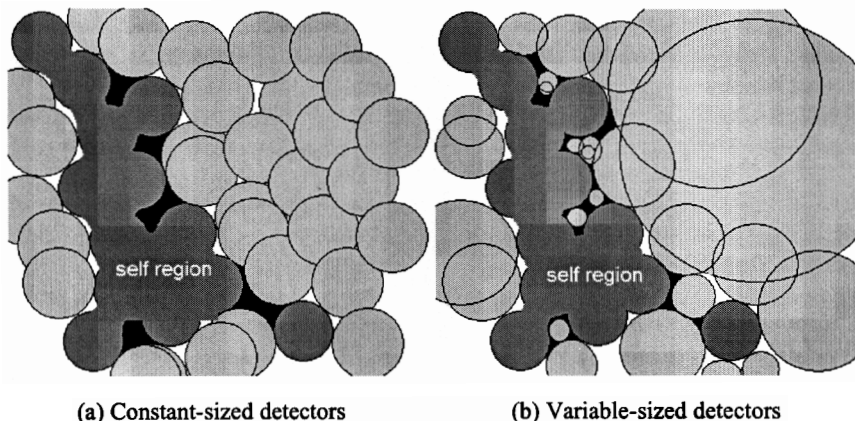
Fig. 1. Main concept of Negative Selection and V-detector
