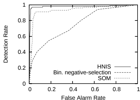
Figure 10. Best ROC curves produced by each method for the Mackey-Glass test data set.
