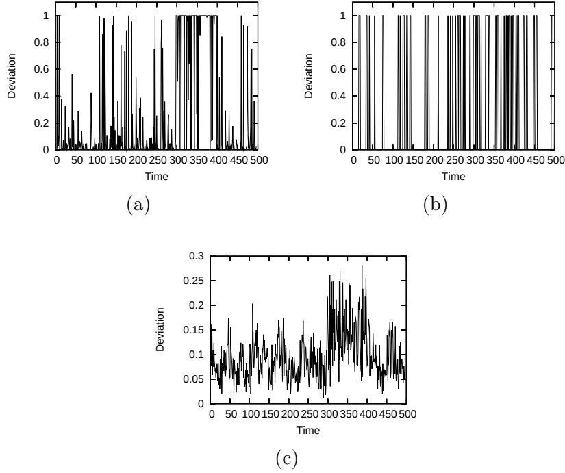
Figure 5. Output value produced by the anomaly function when applied to the Mackey-Glass testing set. (a) HNIS (12 hidden neurons); (b) BNS ( r = 8 , Gray coding); (C) SOM ( 6 \times 6 , D_\infty distance).
