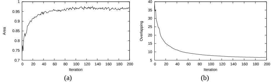
Fig. 4. The RRNS is applied to spread a set of detectors in an unitary square. (a) Progress in the area covered by the detectors. (b) Evolution of the inter-detector overlapping calculated using Equation (9).
