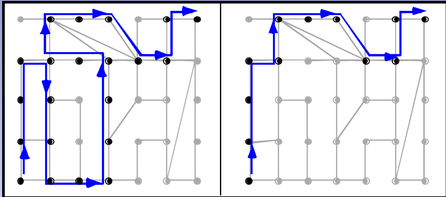
Learning Phase
