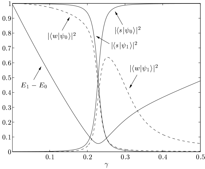
FIG. 2: Energy gap and overlaps for the hypercube with N = 2^{10} = 1024 .
