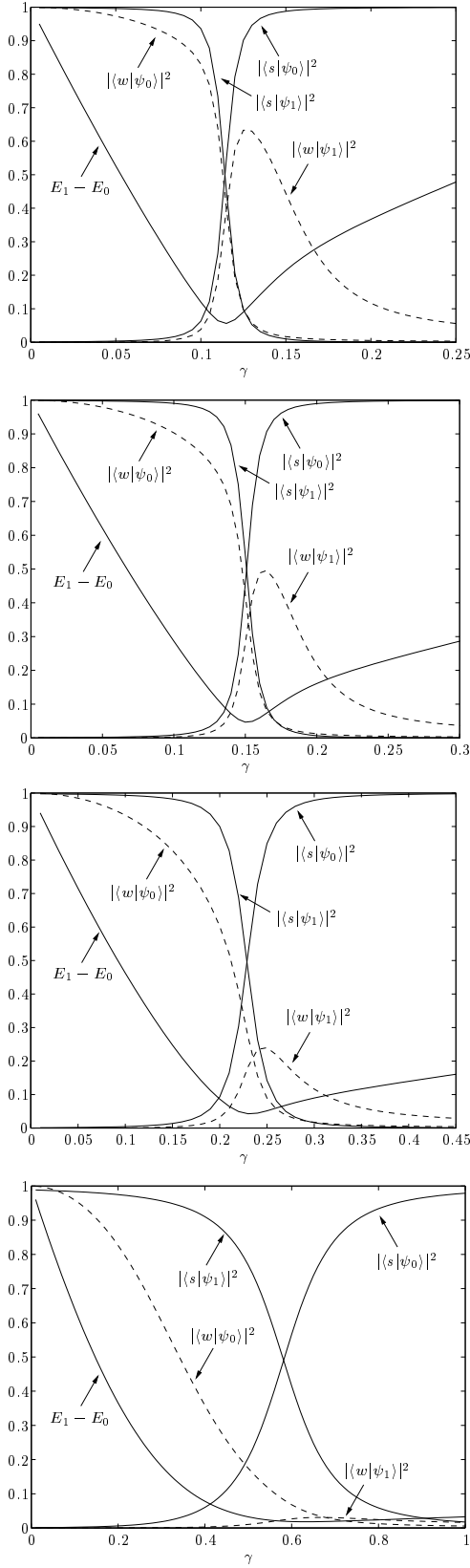
FIG. 3: Energy gap and overlaps for d -dimensional lattices with N \approx 1000 . From top to bottom, d = 5 , N = 4^5 = 1024 ; d = 4 , N = 6^4 = 1296 ; d = 3 , N = 10^3 = 1000 ; d = 2 , N = 32^2 = 1024 .
