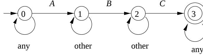
Figure 32: NFA for the episode (A, B, C)
