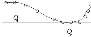
Figure 28: Two examples of queries near a rectangle; note that the query inside the rectangle is actually further from the points on the trail than the query outside the rectangle, but both need to be considered
