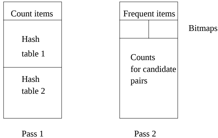
Figure 2: Multiple hash tables memory utilization
