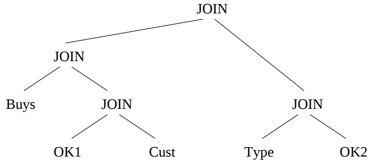
Figure 8: Join order for final step in Fig. 7
