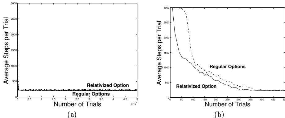
Fig. 6. (a) Comparison of asymptotic performance of the regular and relativized agents on the task in Figure 5. (b) Comparison of initial performance of the two agents on the same task.
