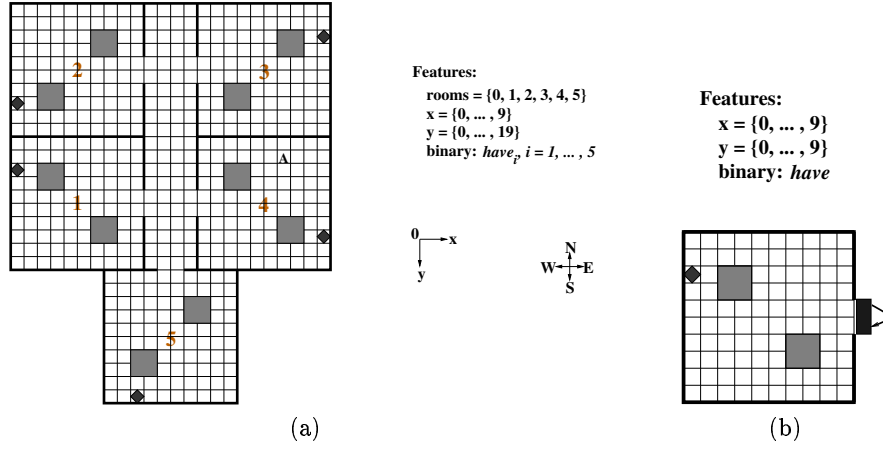
Fig. 2. (a) A simple rooms domain with similar rooms. The task is to collect all 5 objects in the environment. (b) The option MDP corresponding to a get-object-and-leave-room option. See text for full description.
