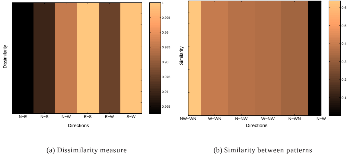
Figure 6.4: (a). Dissimilarity values computed between input patterns representing four orthogonal directions: North , East , South , West . (b). Similarity values between directions situated within a arc circle of 90^\circ : North , North-West , West-North , West . The similarity (or dissimilarity) measure is given by the Euclidian distance between the vectorial representations of the patterns.
