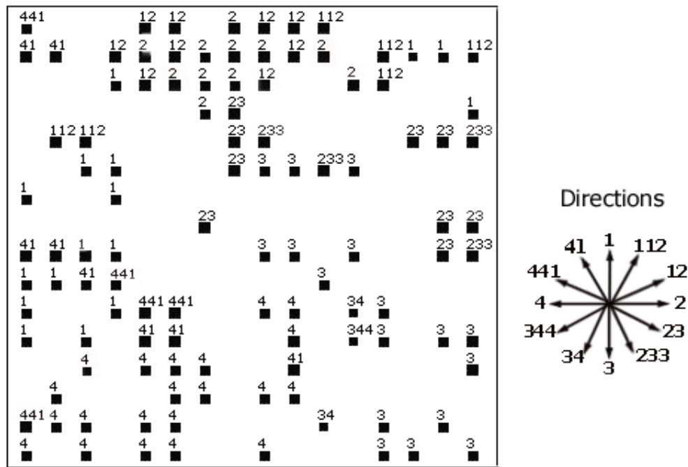
Figure 6.6: Self-organizing map labeled with the winning neurons' preferred directions. The preferred direction is given by the input pattern for which the unit is the best representative, that is, for which it wins most of the times after training has ended.
