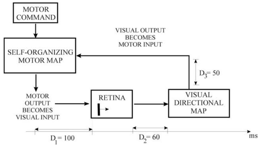
Figure 6.14: Schema of the training procedure used for the alignment of visual and motor directional representations. Note that the motor output becomes visual input and the visual activation is fed back into the motor network. The delay D_1 = 100 ms corresponds to the interval between the time moment when the motor command was issued and the eye starts seeing the arm movement. The delay D_2 = 60 ms represents the time required by the visual input to get from the retina to the visual network. The third value corresponds to the transfer delay from visual area to the motor area of D_3 = 50 ms.
