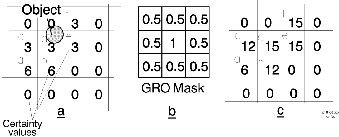
Figure 6: a. In-motion sampling causes sonar readings of an object to be scattered over several cells, resulting in a low OCS. b. 3 \times 3 mask for growth rate operator (GRO). c. With the GRO, OCSs are built up fast and from few readings.
