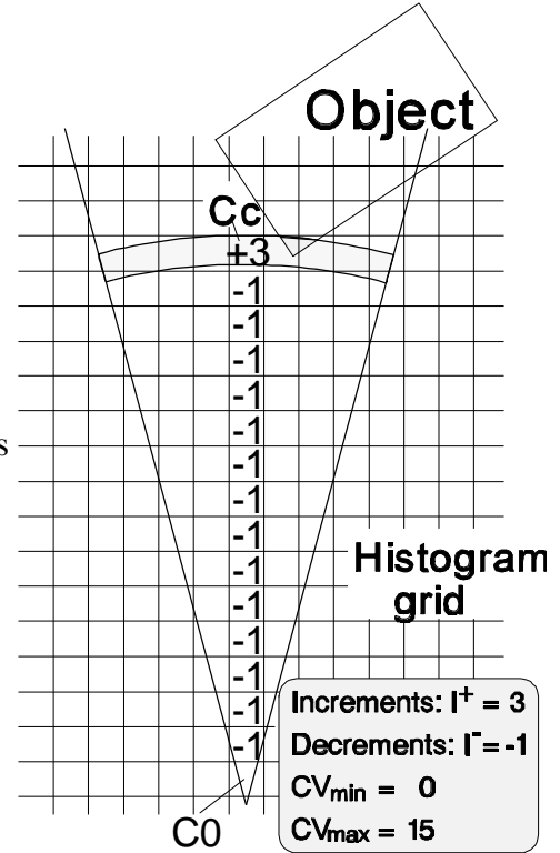
Figure 4: Information on the empty sector between S and A is used to decrement all cells along line C_0 ) C_c .
