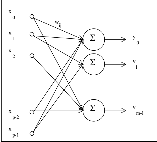
Fig. 2. Detail in PCA network
