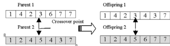
Figure 7. Single-cross-point, value-encoding crossover
