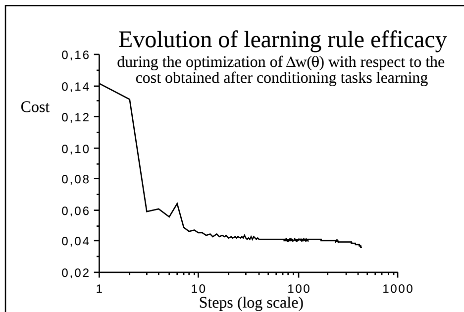
Figure 7: Evolution of the learning rule efficacy
