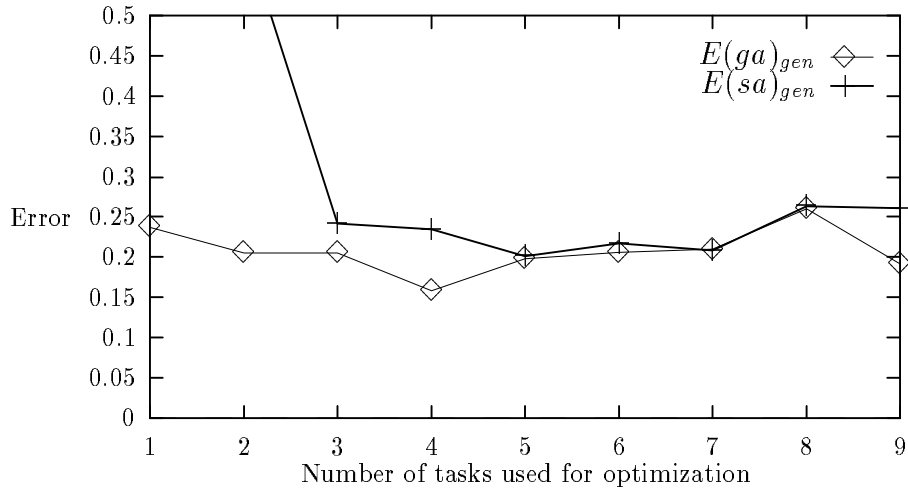
Figure 13: Evolution of generalization error with respect to the optimization method. Here, tasks were linearly separables and the rule had 7 parameters . E(ga)_{gen} represents generalization error with genetic algorithms, and E(sa)_{gen} generalization error with simulated annealing.
