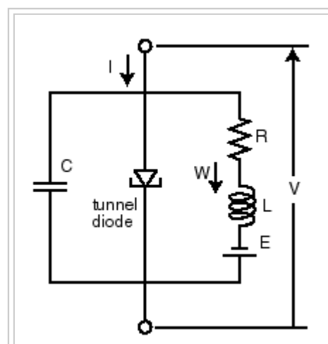
Figure 1: Circuit diagram of the tunnel-diode nerve model of Nagumo et al. (1962).
