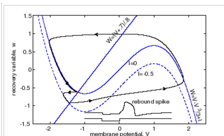
Figure 5: Anodal break excitation (post-inhibitory rebound spike) in the FitzHugh-Nagumo model.
