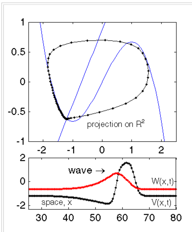
Figure 7: Traveling pulse the FitzHugh-Nagumo reaction-diffusion model. All spatial points are projected onto their V and W coordinates, so that the traveling pulse looks like a circle on the phase plane (notice that because of the diffusion term, the points do not exhibit relaxation oscillations).
