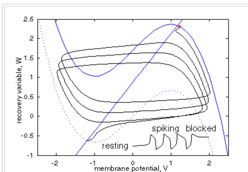
Figure 4: Excitation block in the FitzHugh-Nagumo model.
