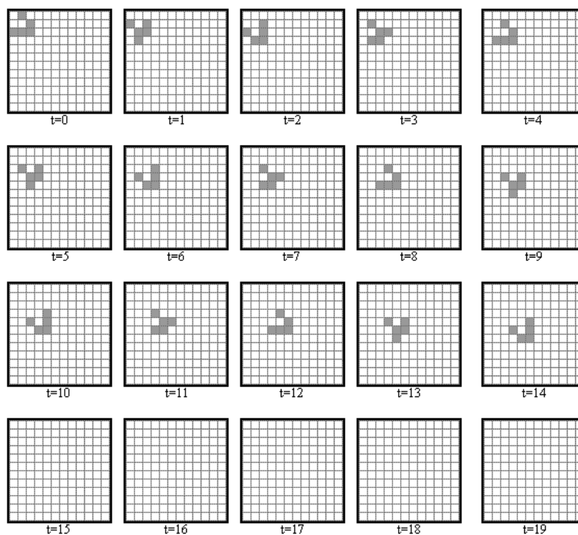
Fig. 2. The “body” ps_{ent}^*(s_t) of the glider (displayed in grey at the first 15 times in the evolution of C^* ). The block does not appear in this figure. For t \geq 15 we have ps_{ent}^*(s_t) = 0 , meaning that the glider is not found on the scene by the observer, since it has been destroyed in the collision against the block visible in Figure 1.
