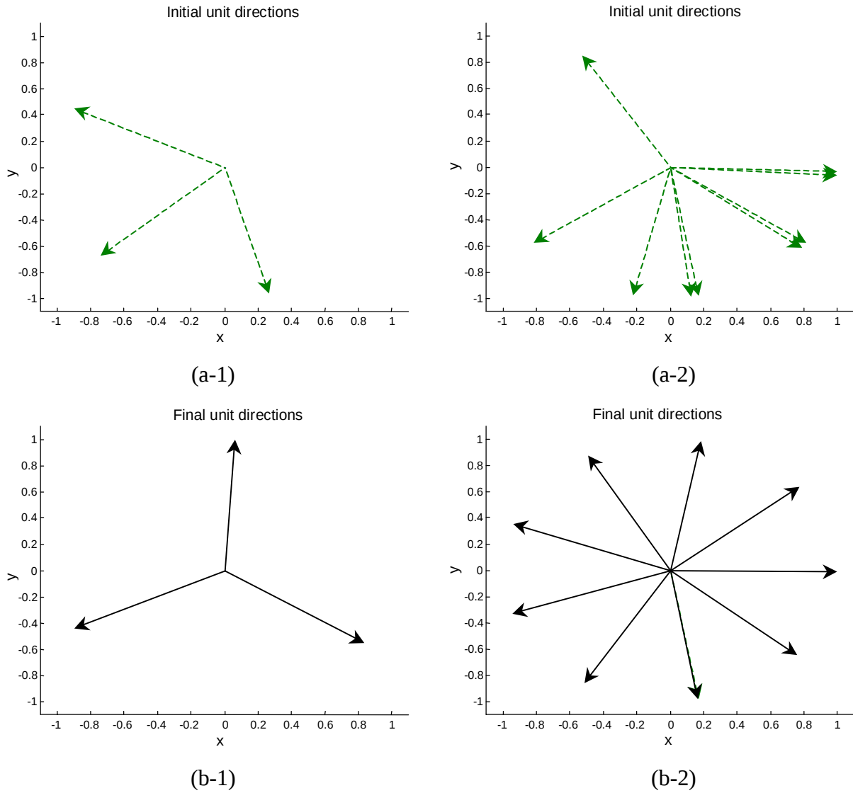
Figure 19: Generation of unit directions using the SA approach applied to Euclidean shape-spaces. The dashed arrows indicate the initial set of vectors (a), and the solid arrows represent the optimized vectors (b). (a-1, b-1) Three vectors ( N = 3 ). (a-2, b-2) Nine vectors ( N = 9 ).
