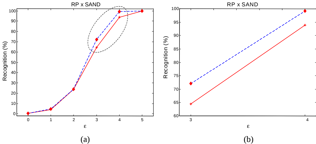
Figure 18: Trade-off between the recognition capability and the affinity threshold \varepsilon . The dashed line corresponds to the proposed method and the solid line corresponds to randomly generated populations, L = 12 , N = 100 , N_{ind} = 14 . (a) \varepsilon \in [0, 5] . (b) Zoom in the circled region of (a), \varepsilon \in [3, 4] .
