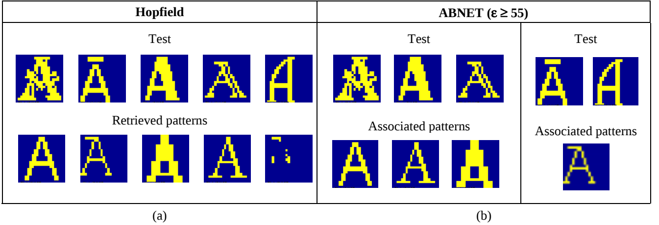
Figure 30: Results obtained for the Hopfield and ABNET algorithms. (a) The Hopfield network could not associate one of the independent patterns with its stored fundamental memories. (b) For \epsilon \geq 55 , the ABNET associated and grouped together two sets of the independent A patterns.
