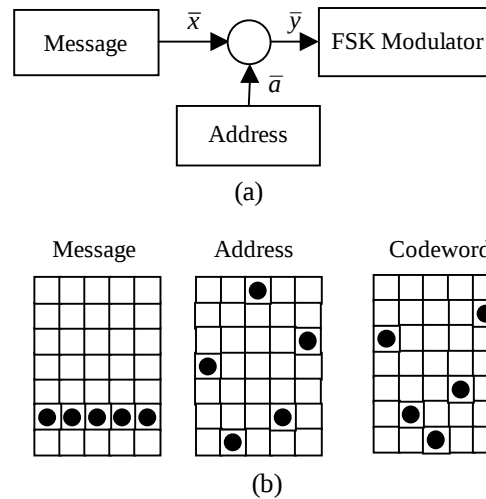
Figure 32: (a) Block diagram for the FH-CDMA multi-level transmitter. (b) Example with Q = 7 and L = 5 : \bar{x} = (1, 1, 1, 1, 1) , \bar{a} = (3, 0, 6, 1, 4) and \bar{y} = (4, 1, 0, 2, 5) .
