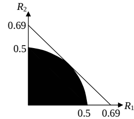
Fig. 7. An achievable region for two-user TDMA system with interference
