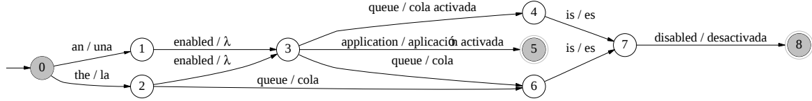
Figure 2: The Finite-State Transducer that is obtained from the bigram of Figure 1
