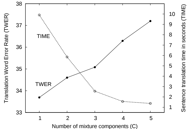
Figure 4: Results obtained with the multiple-model approach and a mixture of multinomials classification model. The plot shows the translation word error rate (TWER) and average sentence translation time (TIME) as a function of the number of mixture components
