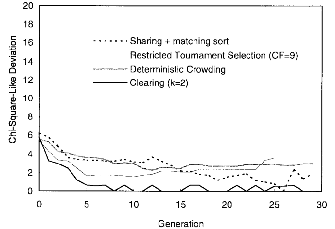
Fig. 14. Chi-square-like deviation of the niching GA's investigated on function F3 . The population size is N = 30 .
