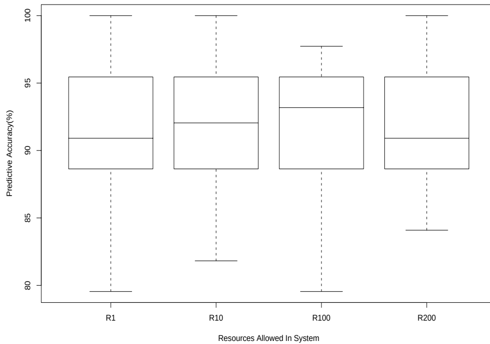
Figure 4.1: Box plot of different numbers of maximum resources allowed in the system
