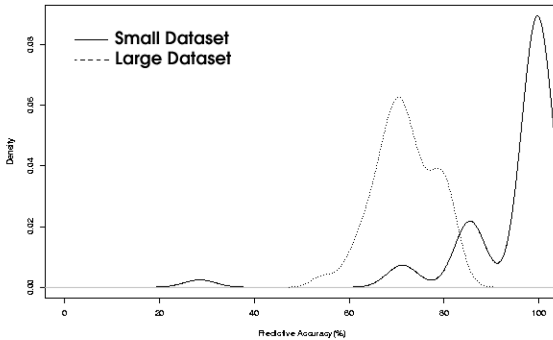
Figure 5.3: Comparison of classifier performance on medium and large document datasets, 64 and 457 documents respectively
