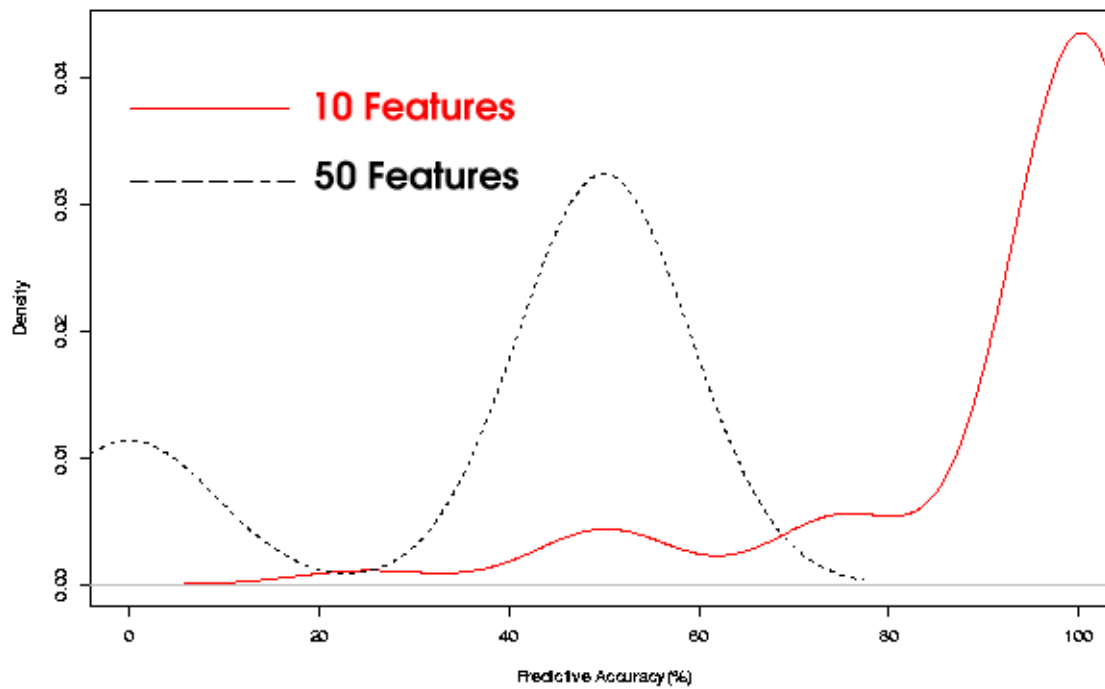
Figure 5.2: Classifier performance for 10 and 50 features, based on a small document dataset of 35 documents
