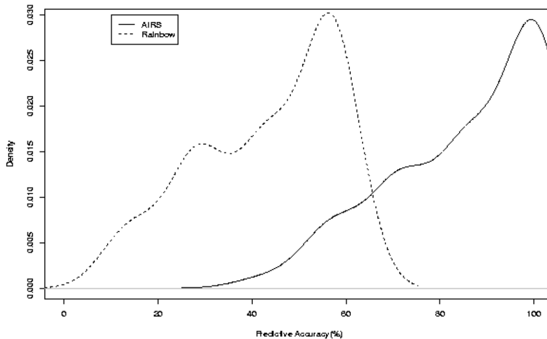
Figure 5.1: A direct comparison between AIRS and the Rainbow Text Classification System
