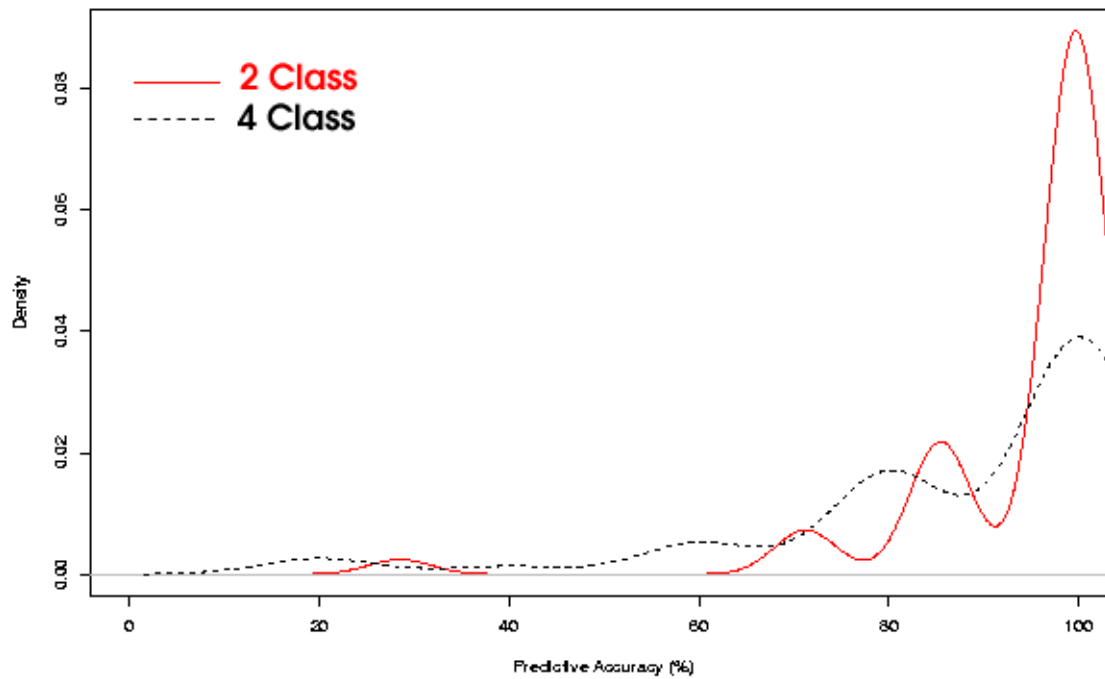
Figure 5.4: Comparison between 2 class and 4 class datasets containing 64 and 80 documents respectively
