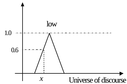
Figure 1: Triangular membership function for a fuzzy set
