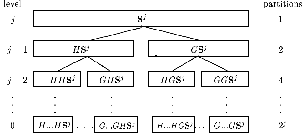
FIG. 3. Application of quadrature filters in wavelet-packet decomposition.
