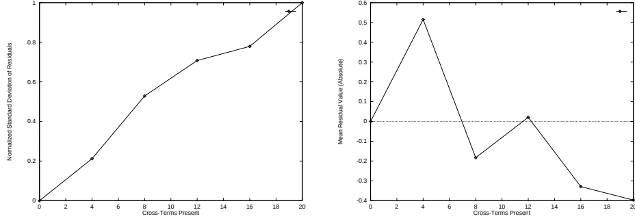
FIG. 6. Residual value standard deviation increases linearly while the mean residual value remains near zero as the number of cross-terms increase
