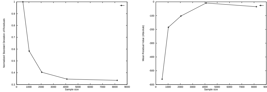
FIG. 7. Global model accuracy increases with sample size
