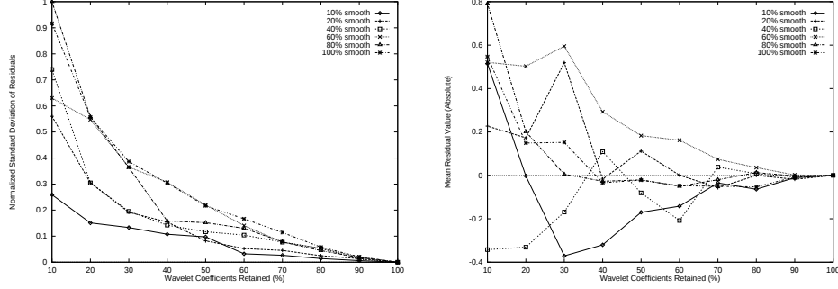
FIG. 5. Model accuracy loss due to retention of fewer wavelet coefficients is reduced as the feature sample characteristics become more consistent with the smoothness of the wavelet function.
