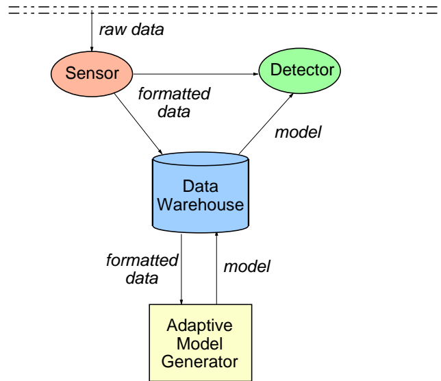
Figure 2. The Architecture of Data Mining-based IDS
