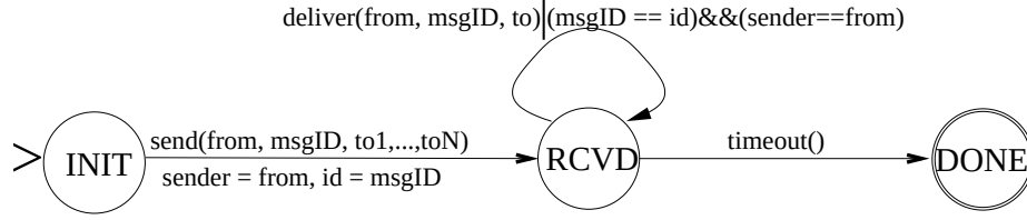
Fig. 1. A State Machine Modeling Email Server Operation
