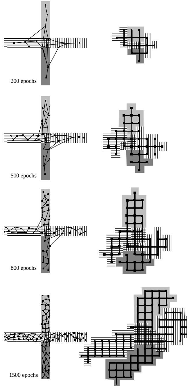
Figure 4.1: Snapshots of the grid evolution for a 2 dimensional cross input. On the left, the weight vectors are plotted on the 2-D input space. On the right, the corresponding grid structure is shown. Shading of the area around a node indicates the arm of the cross where that node's weight vector is located. The four arms are separated in the grid, with a common center.
