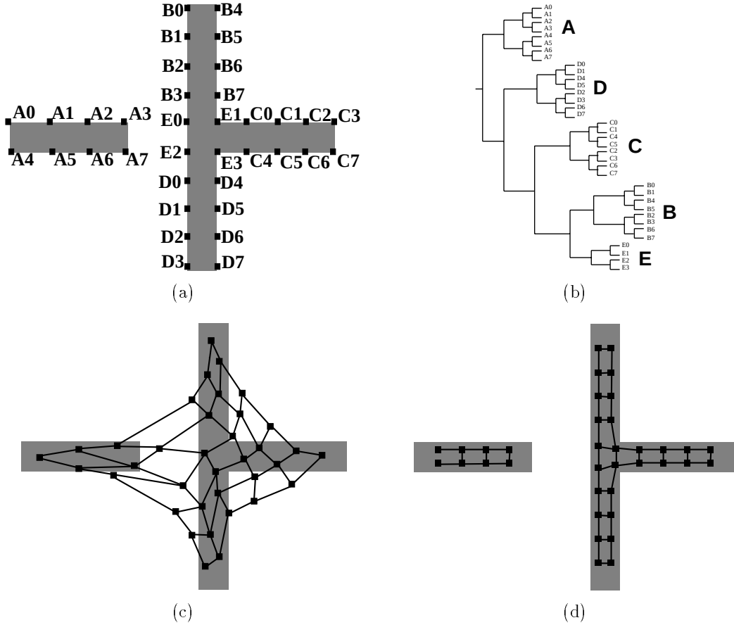
Figure 1.2: Capturing cluster boundaries in a 2-D input space. (a) The input space consists of 36 two-dimensional vectors uniformly distributed in the shaded regions. The vectors were labeled A through E according to the region and numbered. A represents the separated cluster, B, C, and D the connected arms and E the area connecting B, C, and D. (b) The merge clustering representation. The tree structure has captured the clusters in the data, but the overall topology of the data set is not apparent. (c) The self-organizing map representation. The black dots indicate the locations of the network's weight vectors after the map has been organized. Lines indicate network connectivity. Although the map has captured the overall 2-D topology, its connections span the cluster boundaries. Note also that nodes have been allocated to areas where there is no input, representing the structure of the data set inaccurately. (d) A more desirable 2-D network visualization that might be obtained with incremental grid growing. This network has 4 clusters: 3 are connected through a small number of nodes, and the fourth is separate from the others. Note that neither PCA nor MDS is represented here: for 2-D input, these algorithms are not useful.
