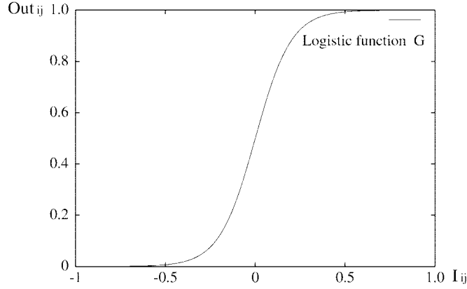
Figure 4. Logistic function
