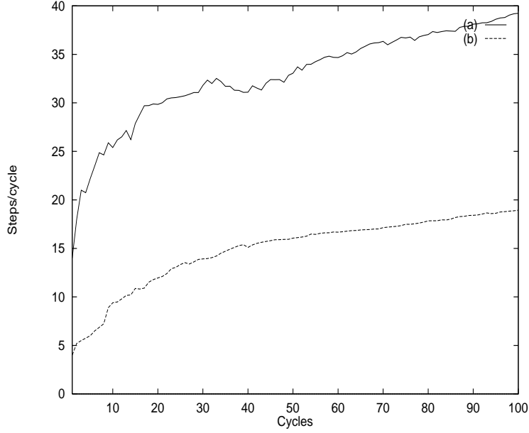
Figure 2: Training Performance
