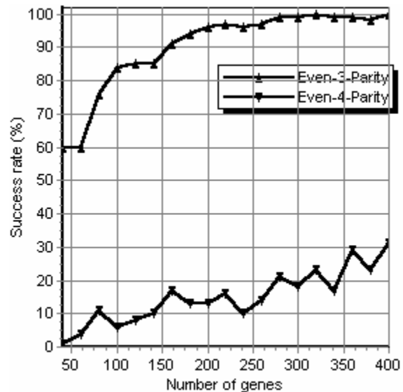
Figure 1: The relationship between the success rate and the number of genes in a MEP chromosome. Results are summed over 100 runs.
