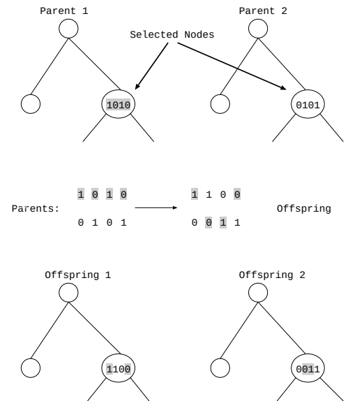
Figure 3: Uniform crossover on the sub-symbolic representation.
